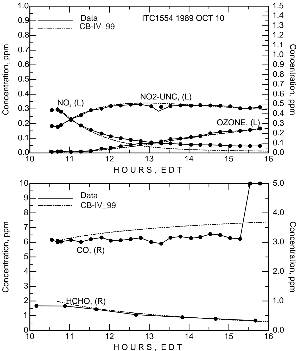
Figure C-22. Simulation results for the October 10, 1989 HCHO/NO x experiment (ITC1554).
