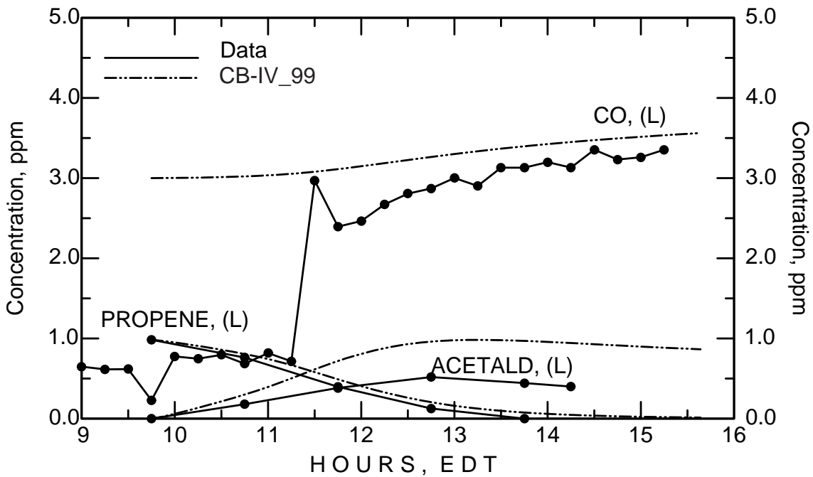
Figure C-29. Simulation results for the October 5, 1989 propene/NO x experiment (ITC1550).
