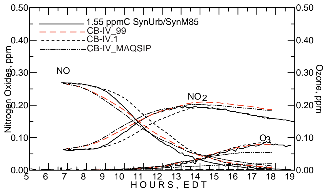
Figure C-15. August 30, 1991 Urban Mix/NO x experiment simulation comparing three models.
