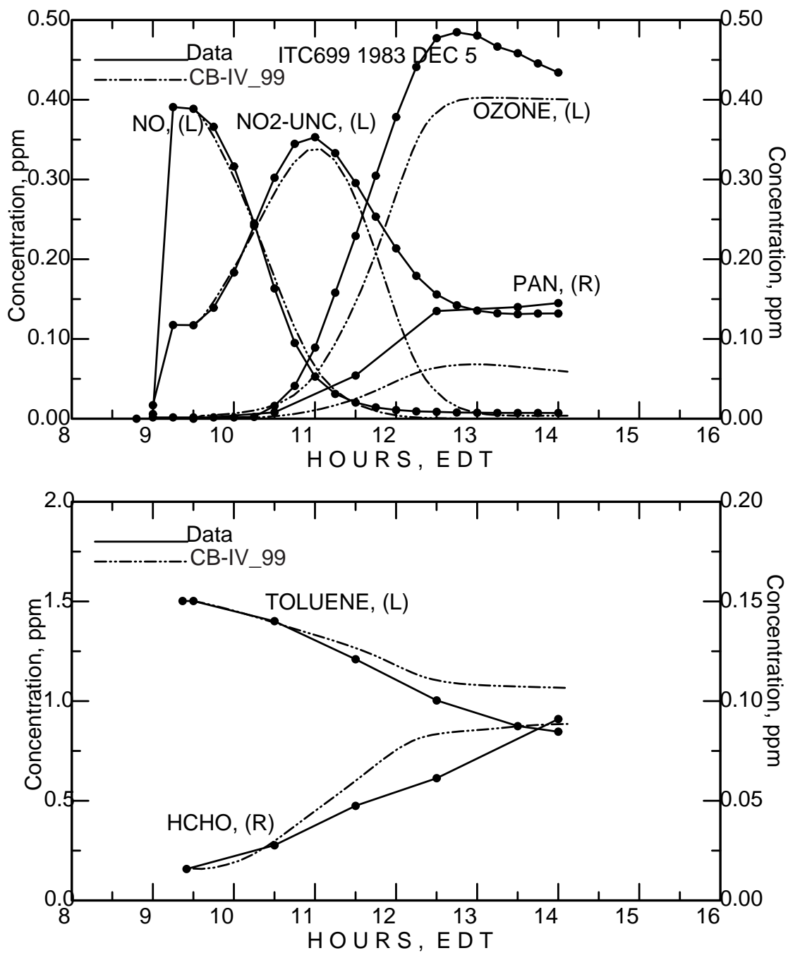
Figure C-30. Simulation results for the December 5, 1983 toluene/NO x experiment (ITC699).
