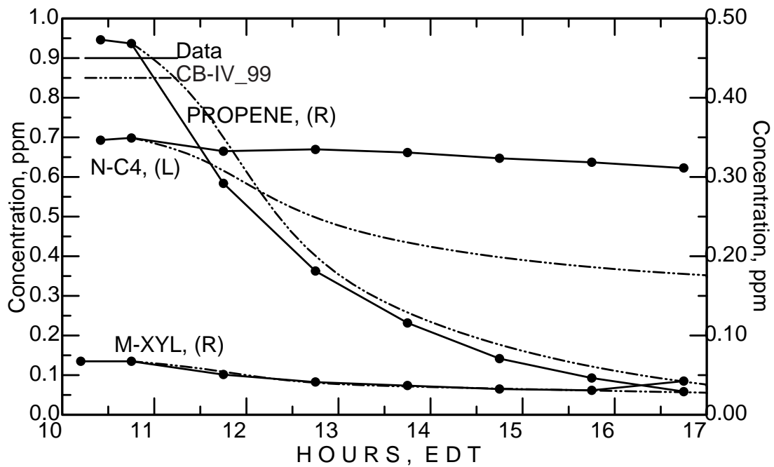
Figure C-34. Simulation results for the February 8, 1983 mini-surrogate/NO x experiment (ITC585).
