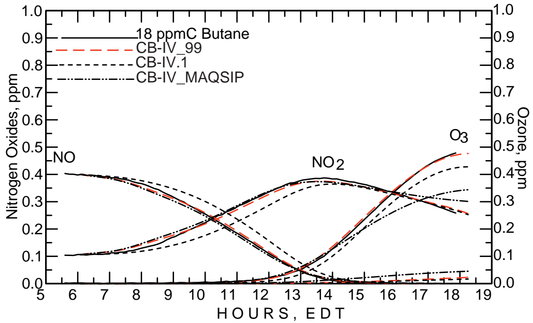
Figure C-10. May 23, 1992 butane/NO x experiment simulation comparing three models.
