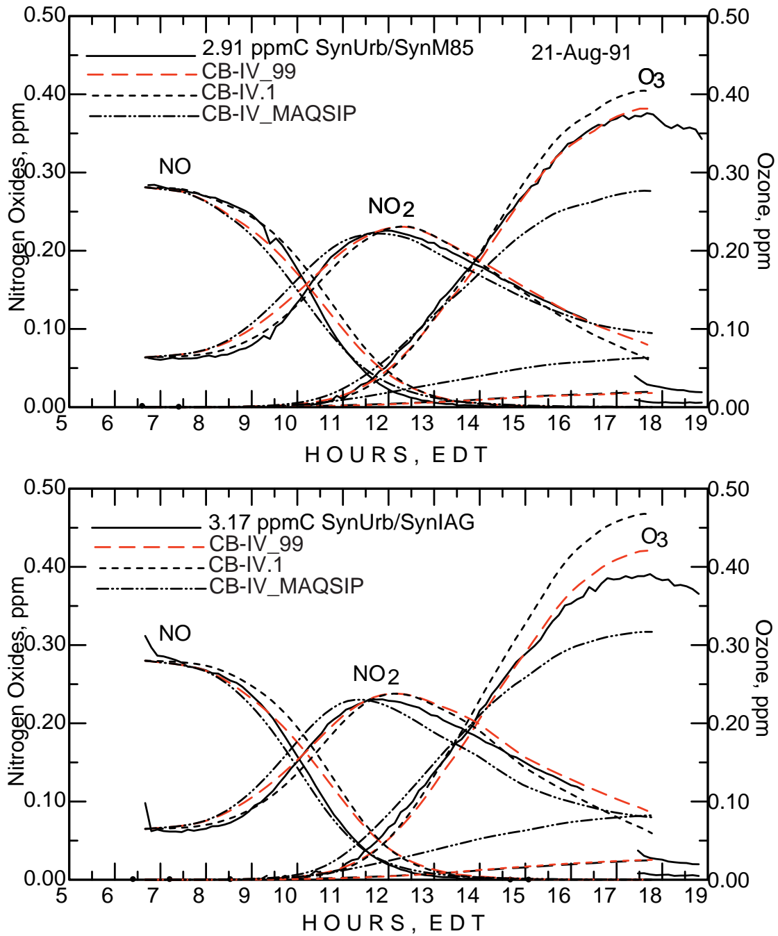
Figure C-14. August 21, 1991 Urban Mix/NO x experiment simulation comparing three models.
