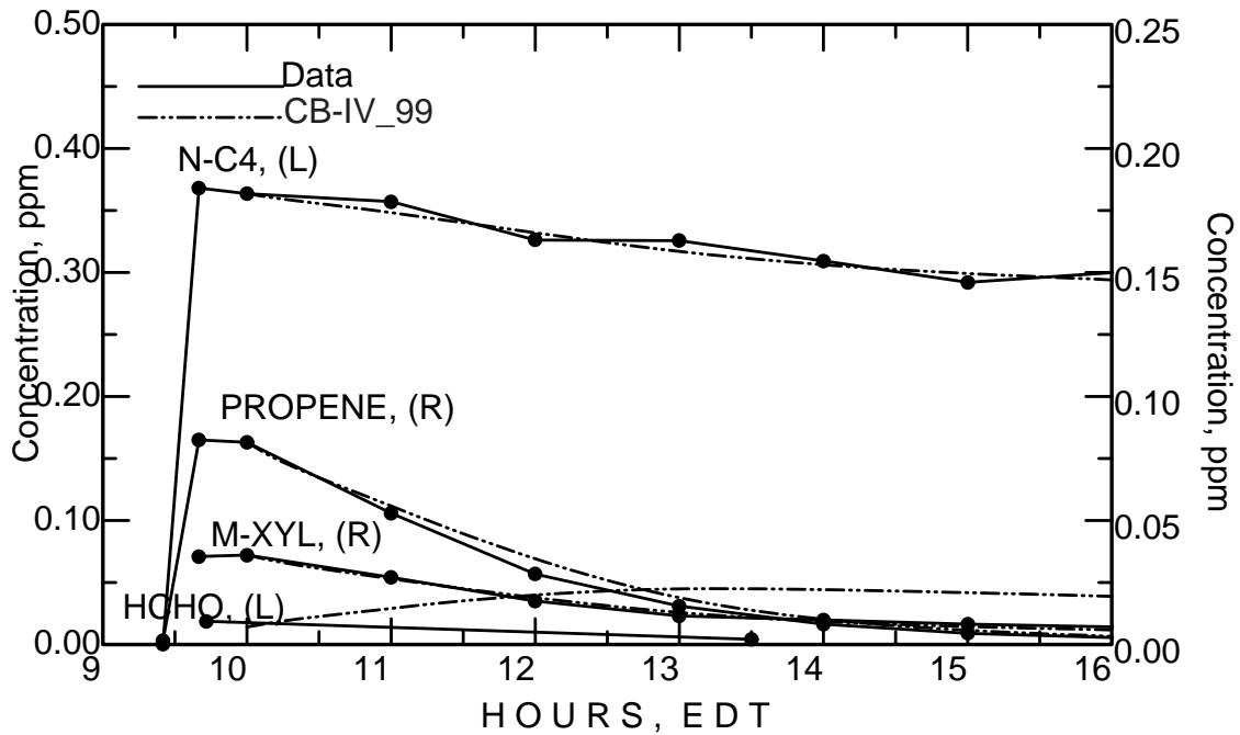
Figure C-31. Simulation results for the February 16, 1982 mini-surrogate/ \text{NO}_x experiment (ITC440).
