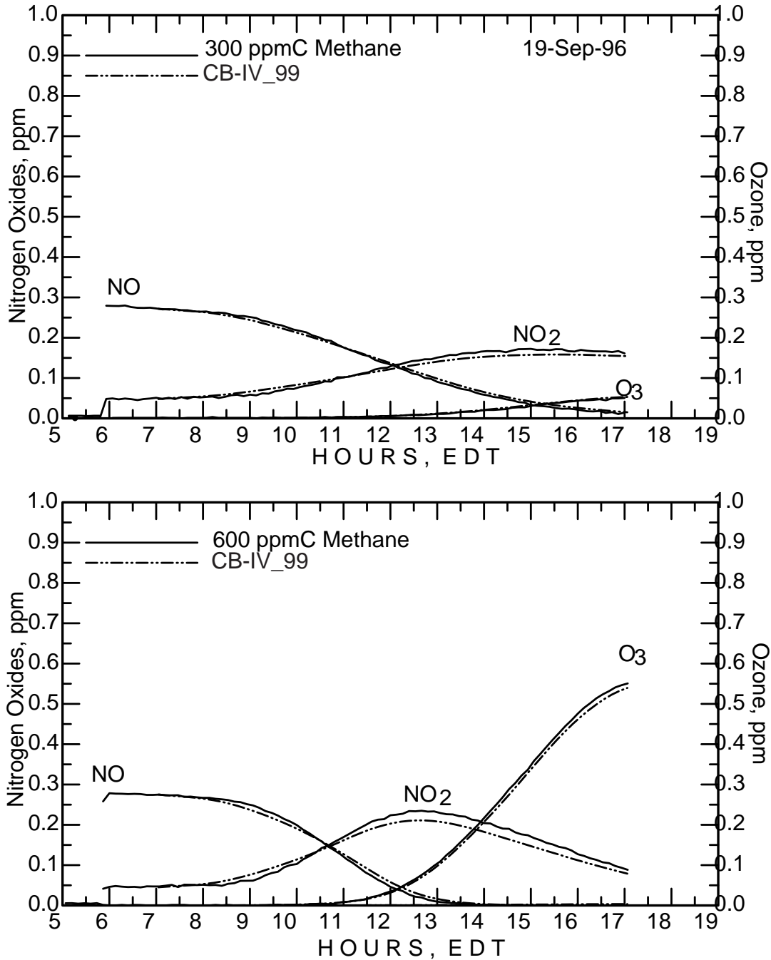
Figure C-1. Simulation results for the September 19, 1996 methane/NO x experiment - O 3 and NO x .
