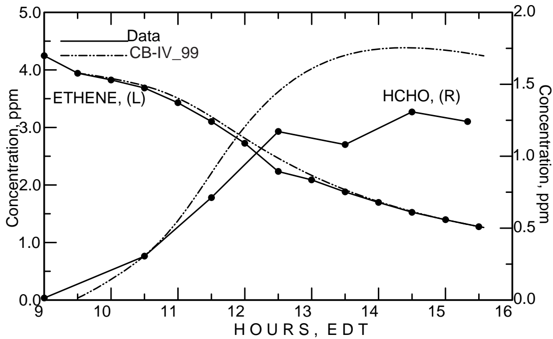
Figure C-26. Simulation results for the March 13, 1986 ethene/NO x experiment (ITC926).
