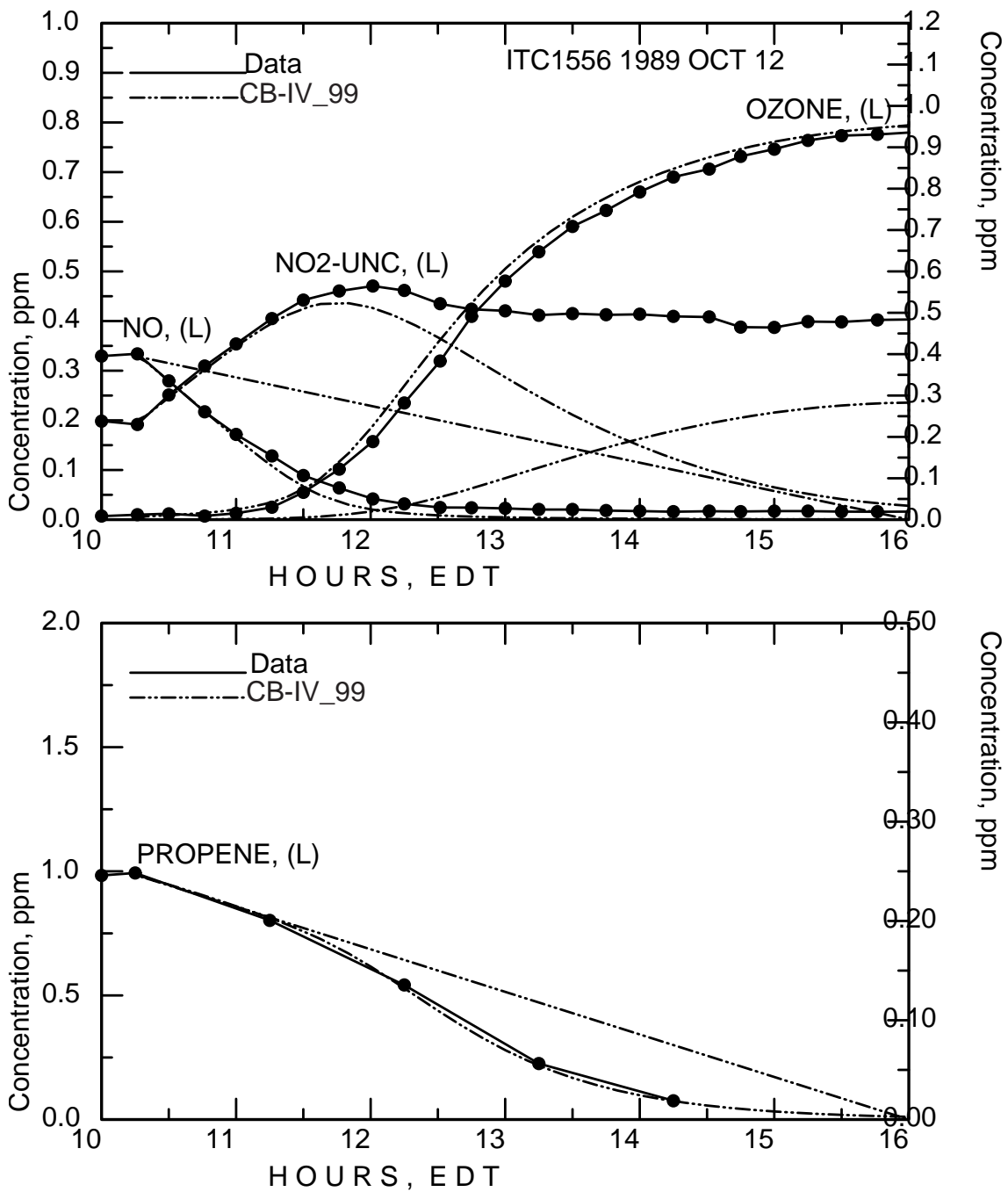
Figure C-28. Simulation results for the October 12, 1989 propene/NO x experiment (ITC1556).
