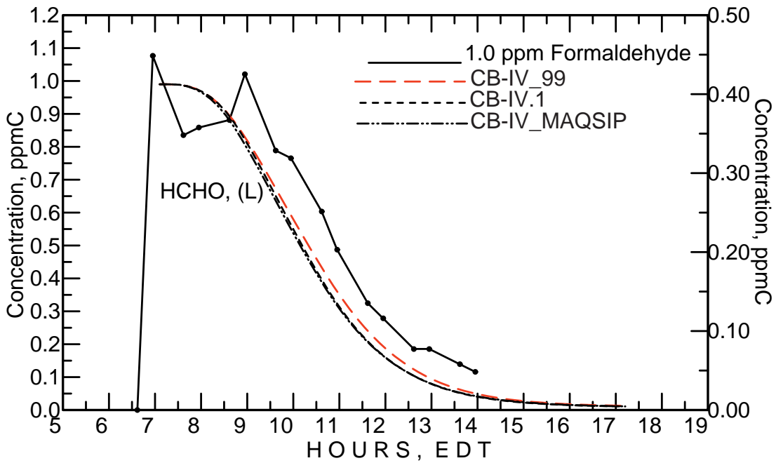
Figure C-6. September 23, 1996 HCHO/NO x experiment simulation comparing three models (HC).
