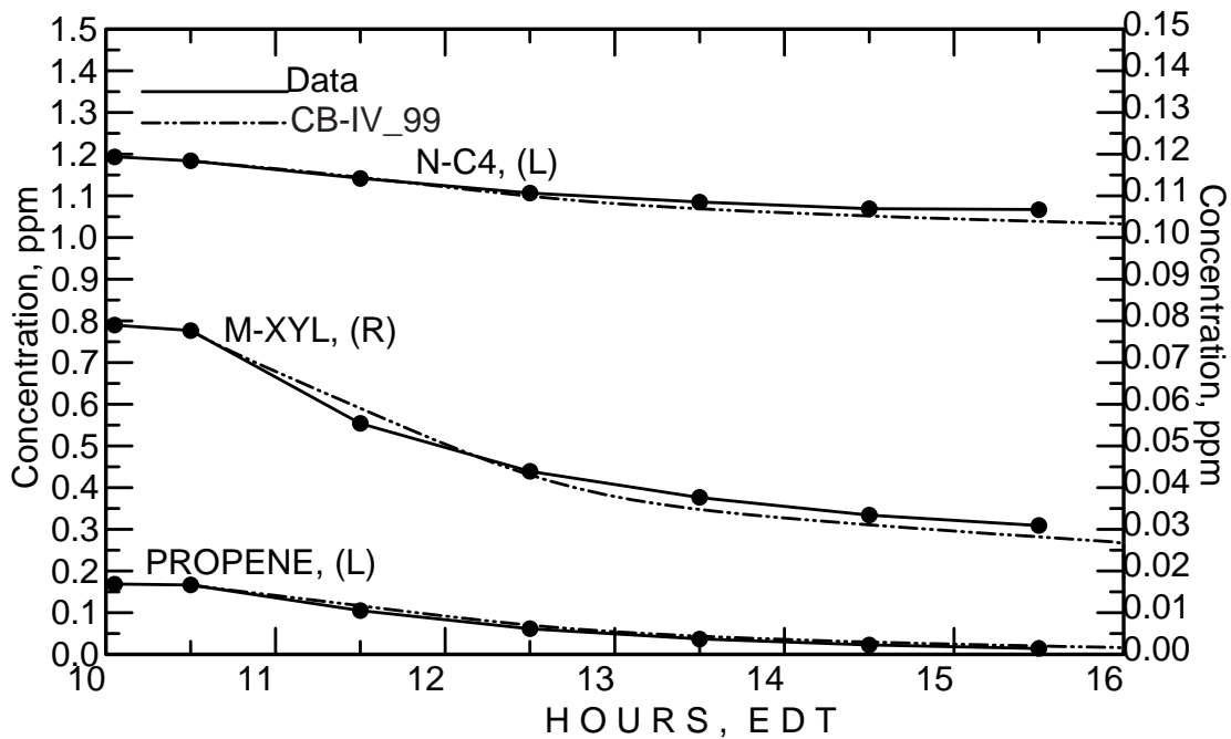
Figure C-33. Simulation results for the April 29, 1982 mini-surrogate/ \text{NO}_x experiment (ITC488).
