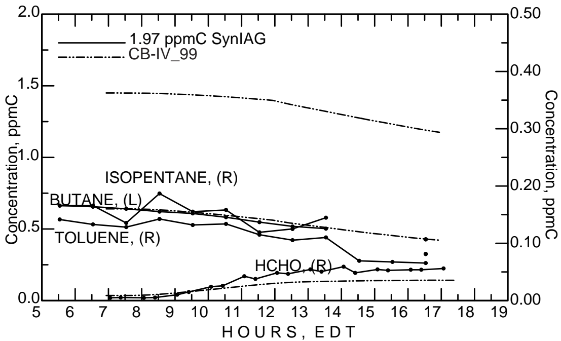
Figure C-13. Simulation results for the Sept. 10, 1991 Urban Mix/NO x experiment – HC.
