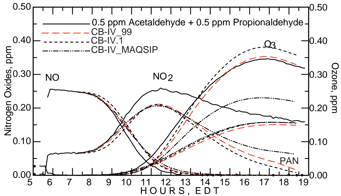
Figure C-7. October 4, 1996 aldehyde/NO x experiment simulation comparing three models.
