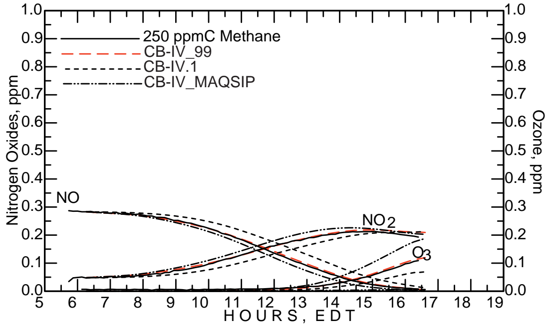
Figure C-3. July 21, 1991 Methane/NO x experiment simulation comparing three models.
