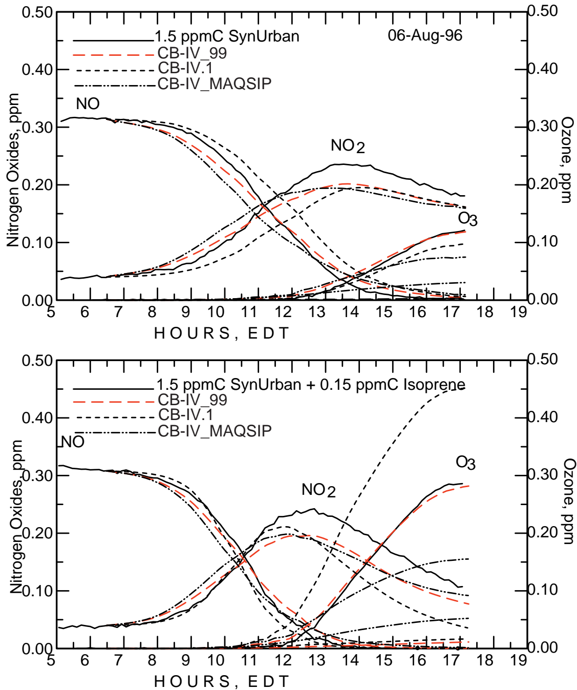
Figure C-20. August 6, 1996 Isoprene MIR experiment simulation comparing three models.
