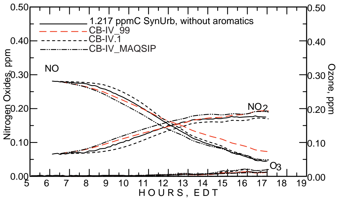
Figure C-16. August 11, 1992 Urban Mix/NO x experiment simulation comparing three models.
