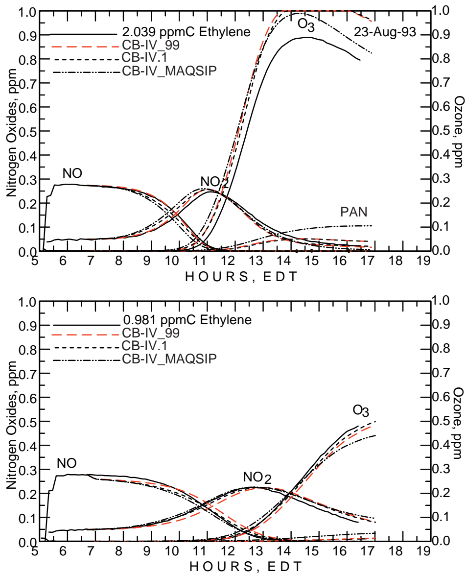
Figure C-8. August 23, 1993 ethene/NO x experiment simulation comparing three models.
