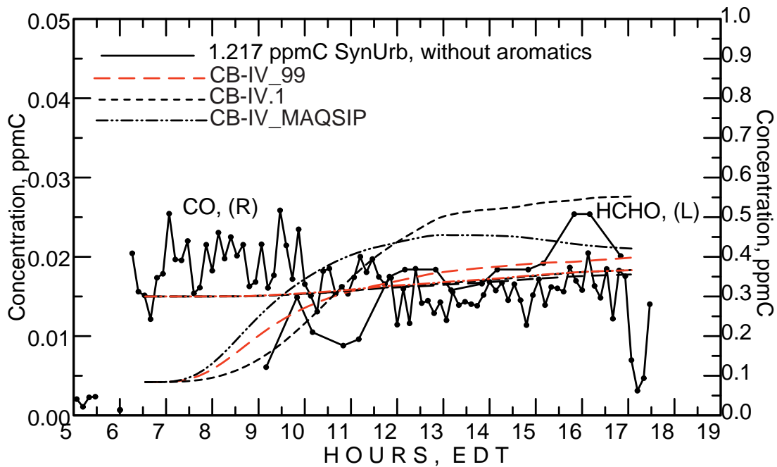
Figure C-17. August 11, 1992 Urban Mix/NO x experiment simulation comparing three models (HC).
