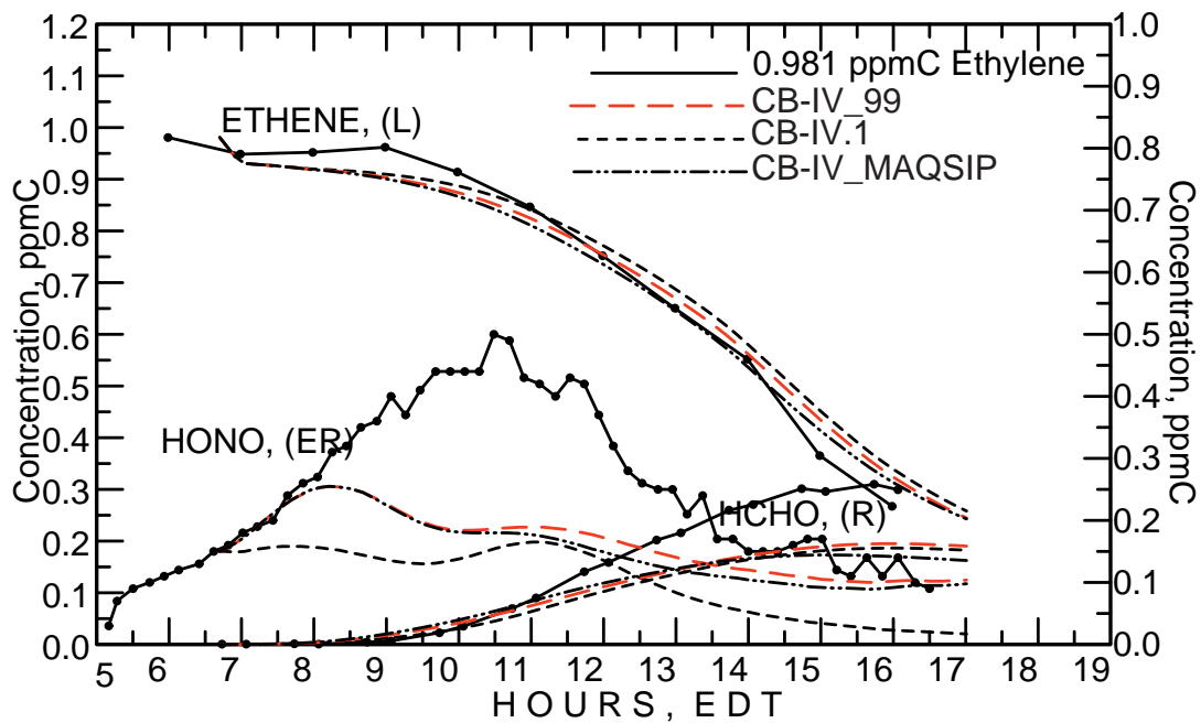
Figure C-9. August 23, 1993 ethene/NO x experiment simulation comparing three models (HC).
