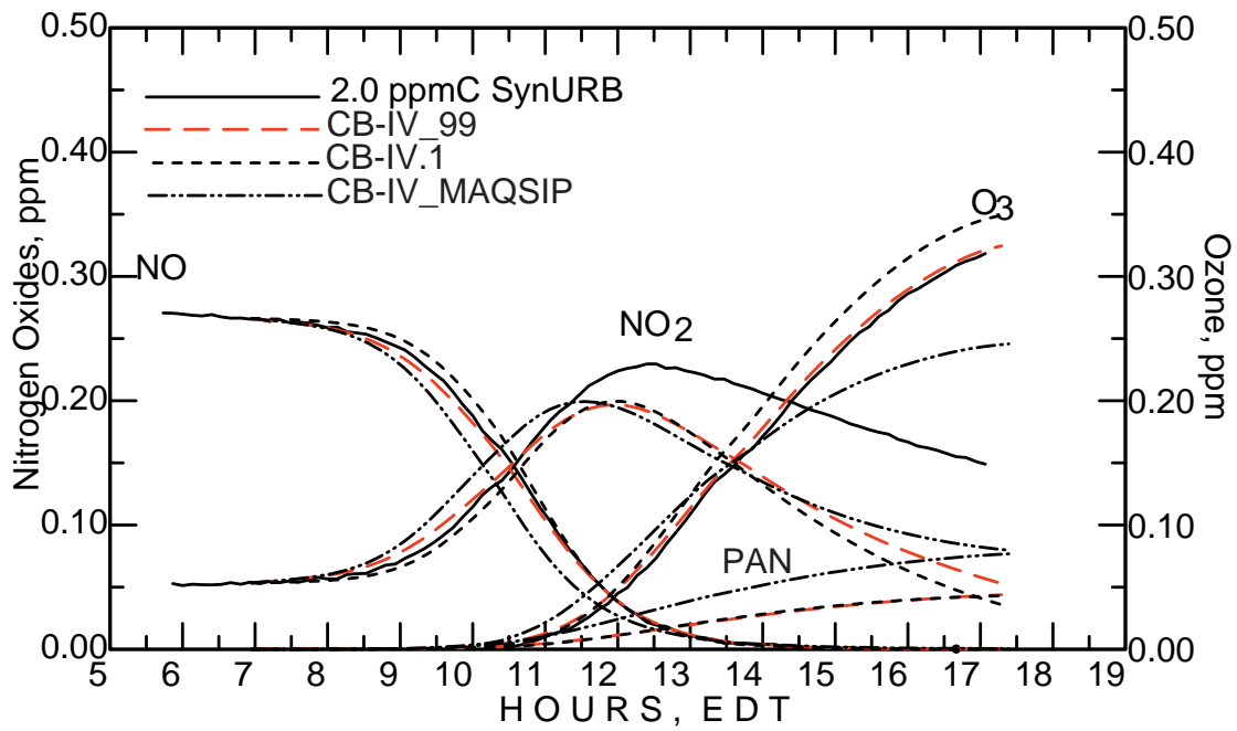
Figure C-18. September 12, 1994 Urban Mix/NO x experiment simulation comparing three models.
