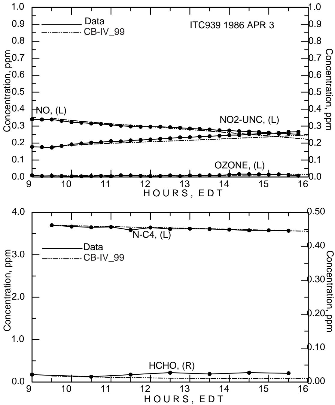
Figure C-23. Simulation results for the April 3, 1986 n-Butane/NO x experiment (ITC939).
