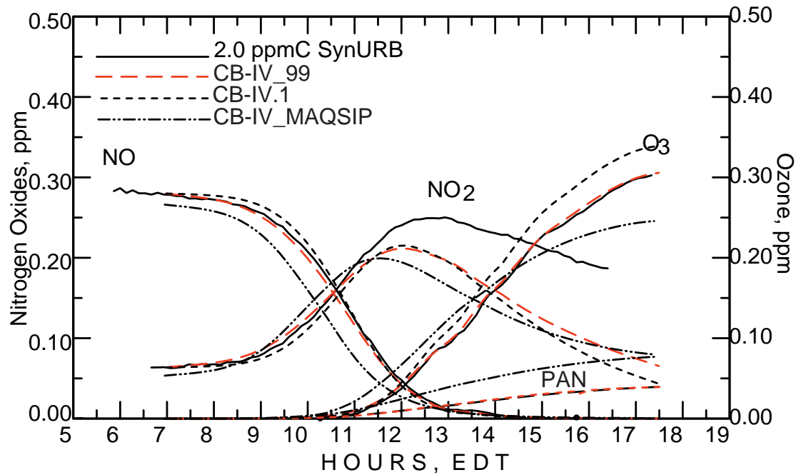
Figure C-19. September 15, 1994 Urban Mix/NO x experiment simulation comparing three models.
