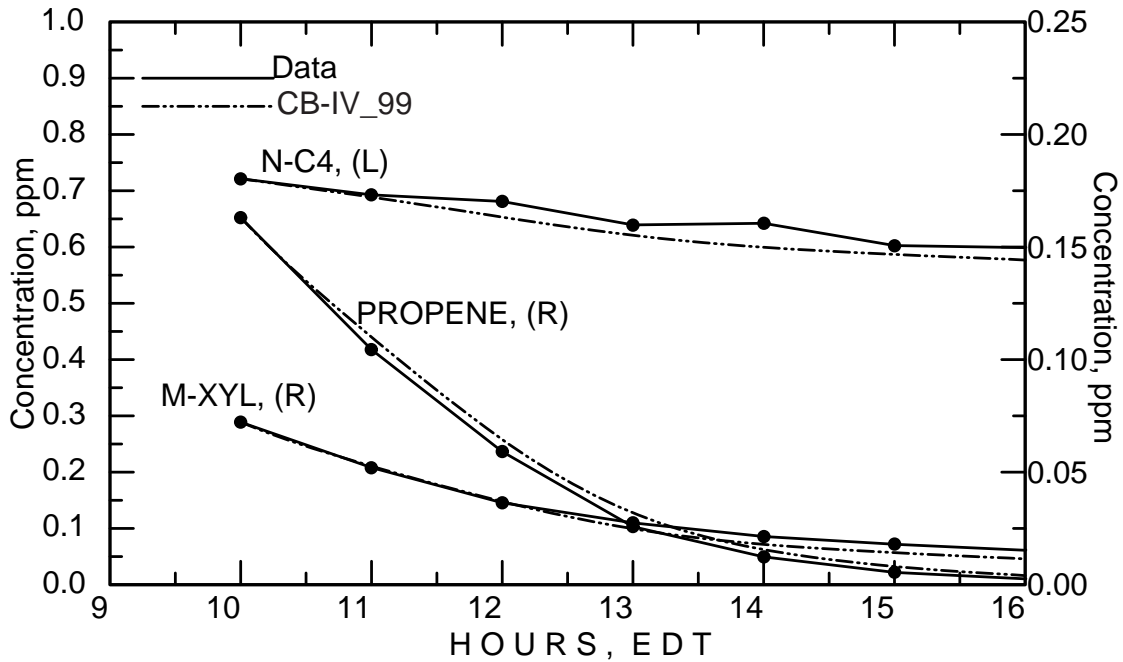
Figure C-32. Simulation results for the February 18, 1982 mini-surrogate/NO x experiment (ITC442).
