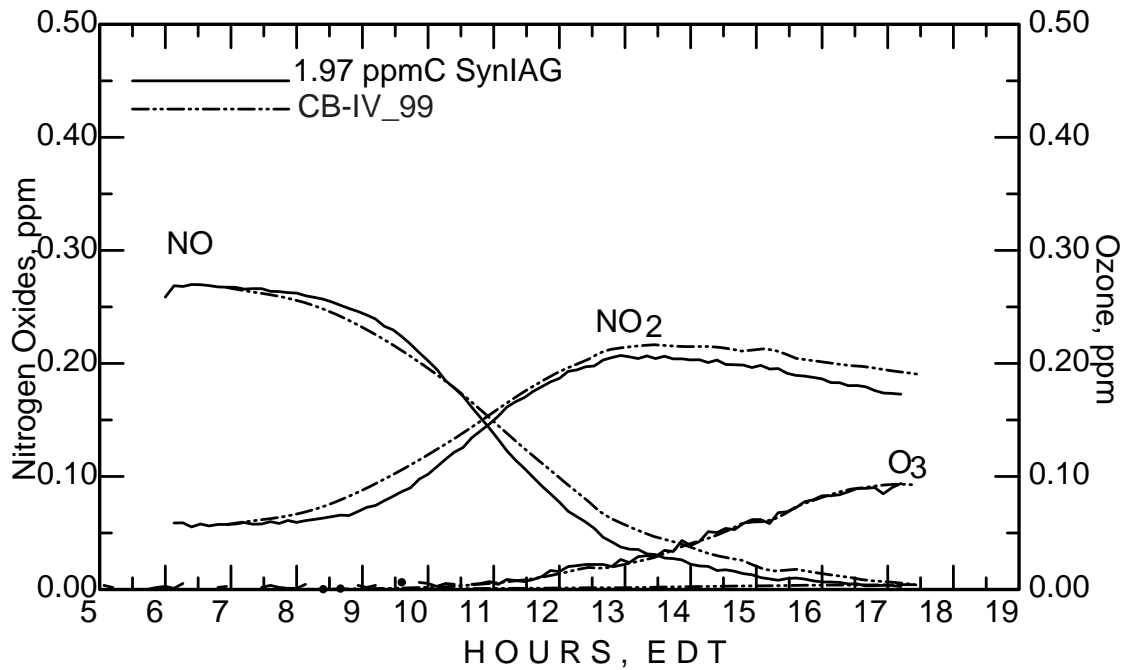
Figure C-12. Simulation results for the Sept. 10, 1991 Urban Mix/NO x experiment – O 3 and NO x .
