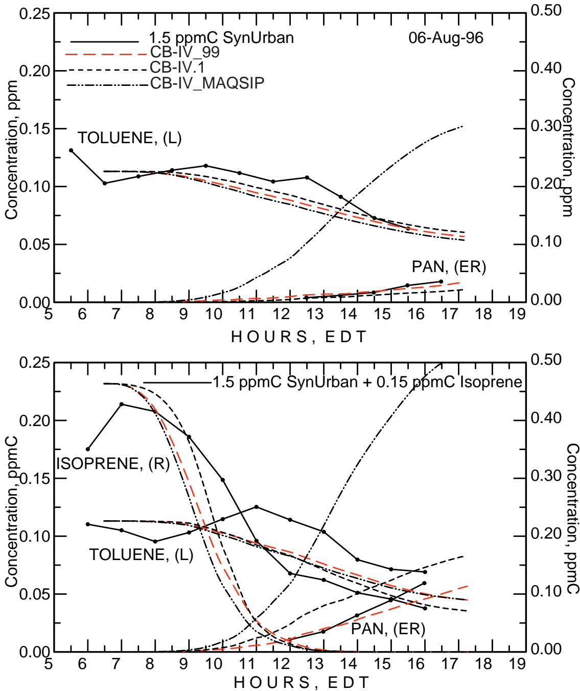
Figure C-21. August 6, 1996 isoprene MIR experiment simulation comparing three models.
