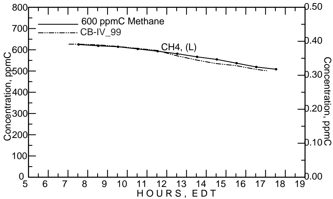
Figure C-2. Simulation results for the September 19, 1996 methane/NO x experiment – HC.
