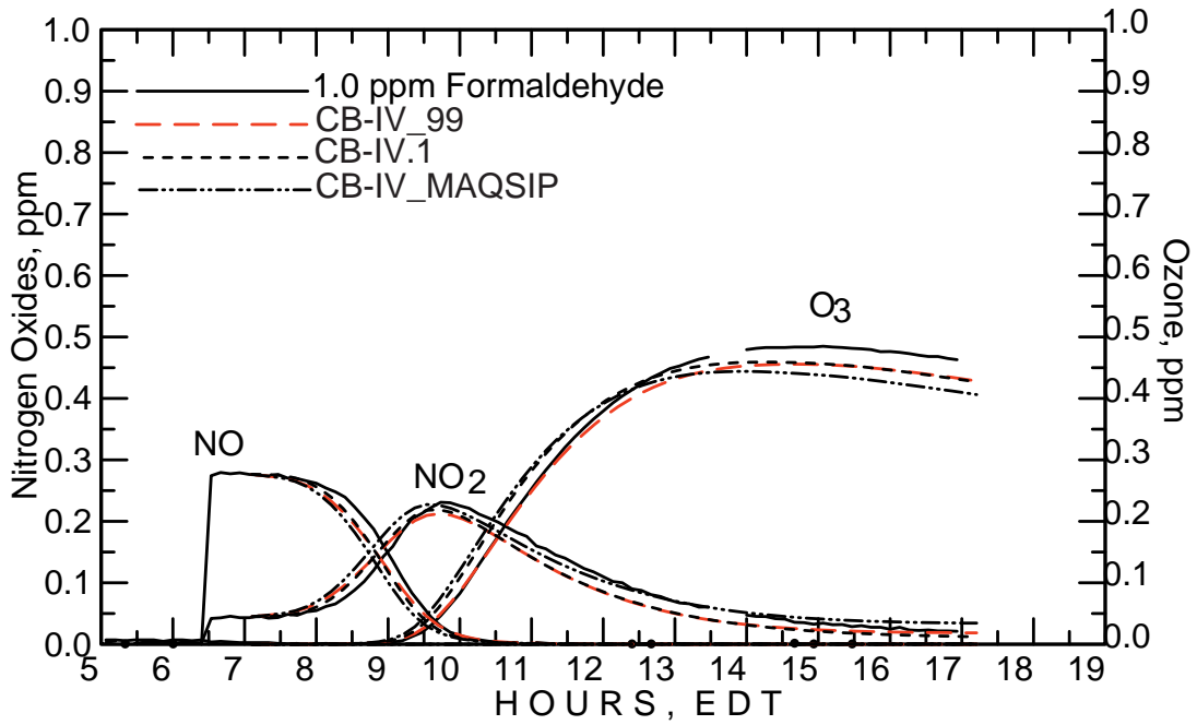
Figure C-5. September 23, 1996 HCHO/NO x experiment comparison of three models.
