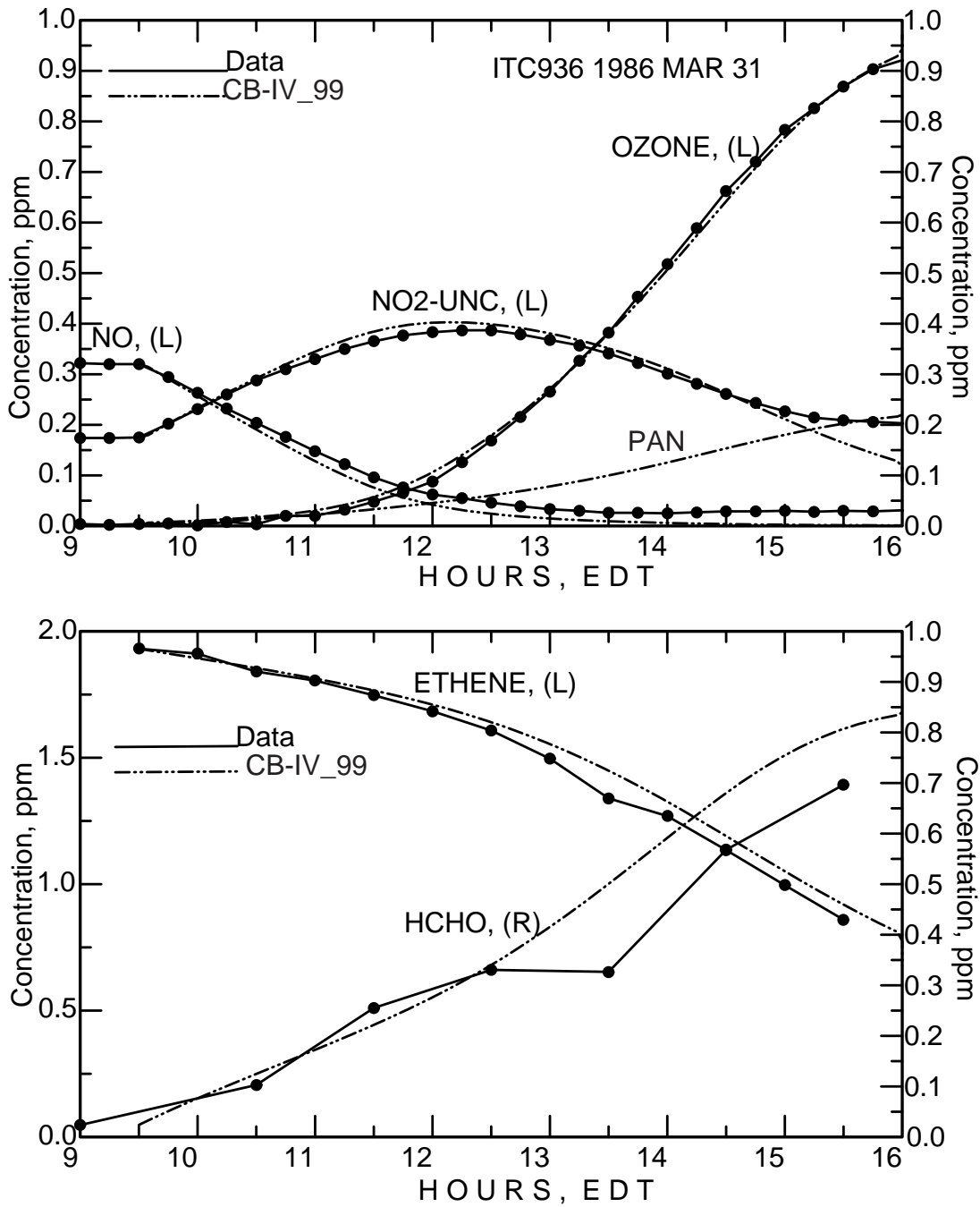
Figure C-27. Simulation results for the March 31, 1986 ethene/NO x experiment (ITC936).
