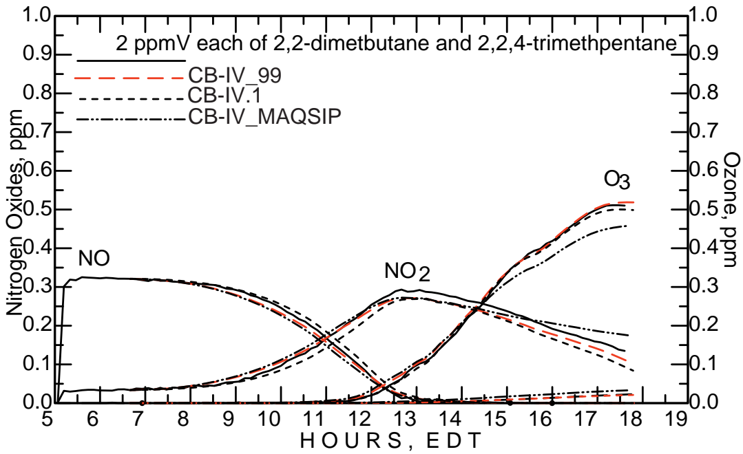
Figure C-11. August 20, 1996 paraffin/NO x experiment comparing three models.
